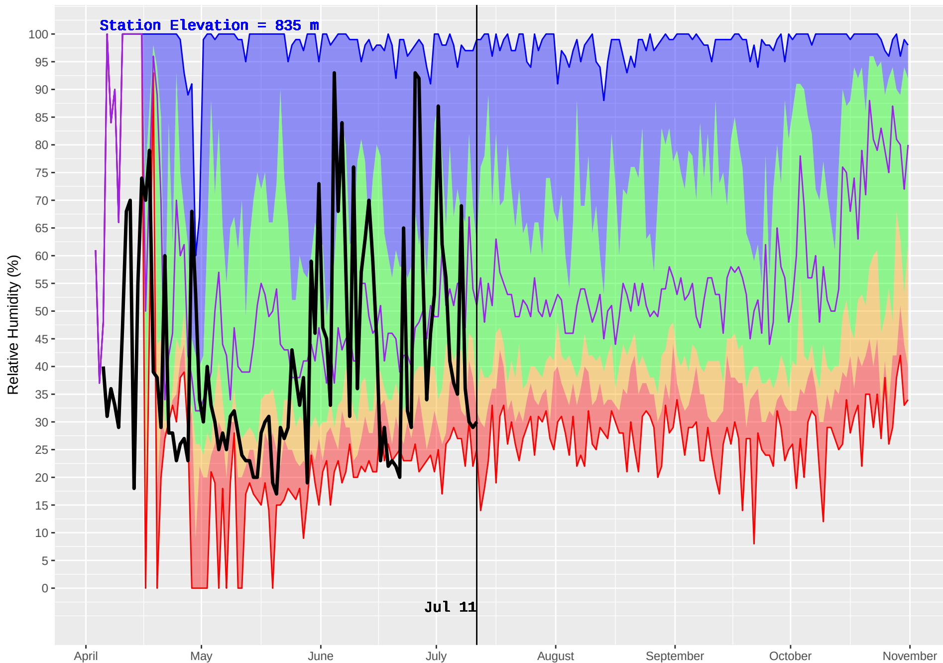
SILVER (120) : Historical (1986–2016) and Current (2018) Noon Relative Humidity
