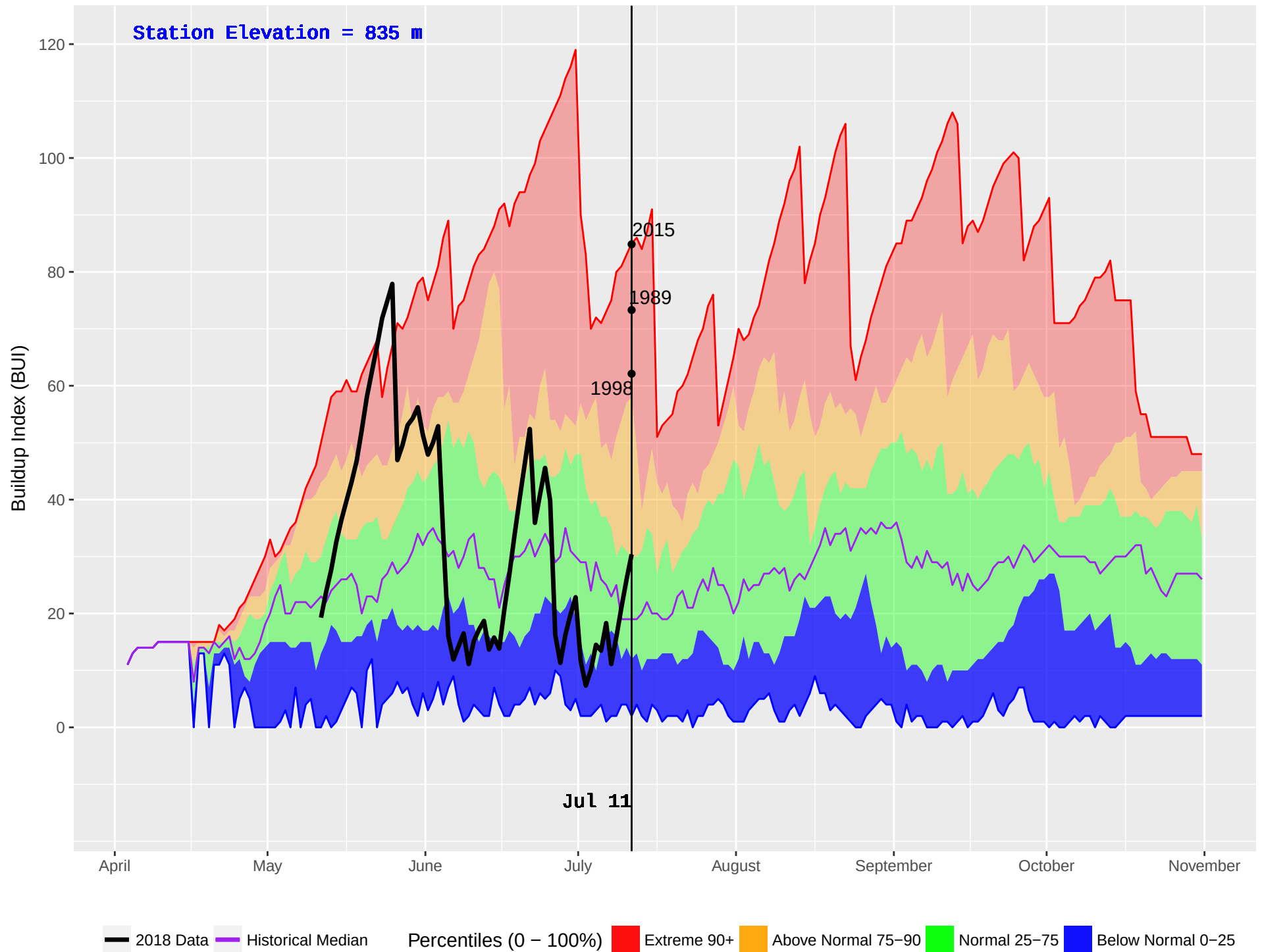
SILVER (120) : Historical (1986–2016) and Current (2018) Noon Buildup Index (BUI)
